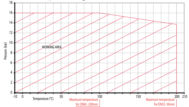
Pressure/Temperature Diagram
