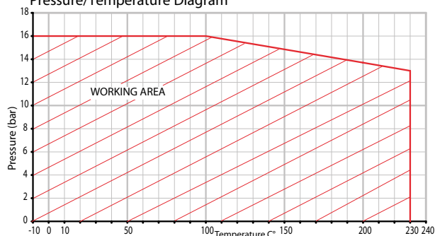
Pressure/Temperature Diagram
