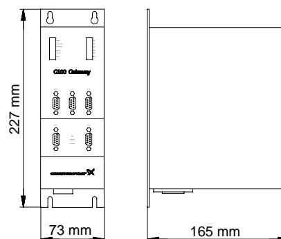
Fig. 21 Dimensional sketch
