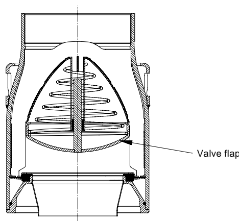
Fig. 5 Non-return valve
